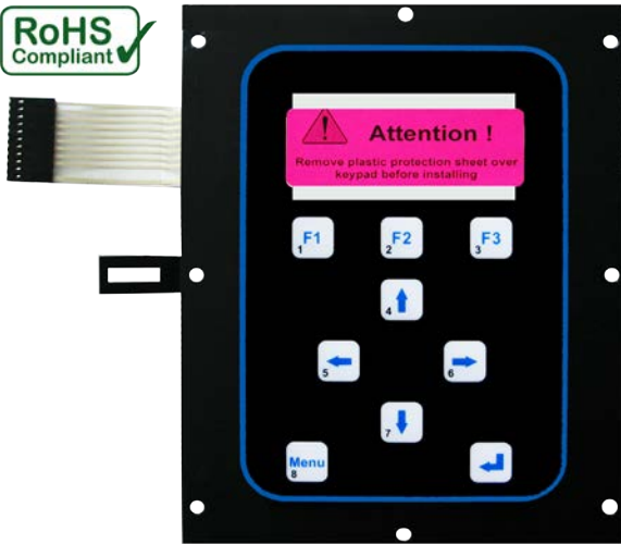
Part # MAG-KEYPAD-OEM-232
