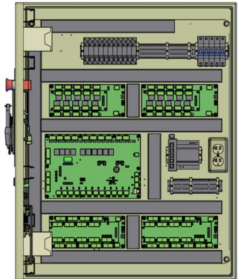
Front Open View
