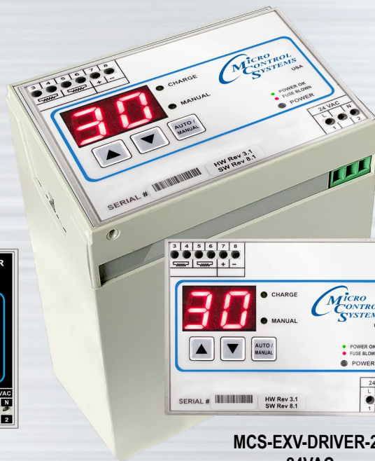
MCS-EXV-DRIVER 110-240VAC
