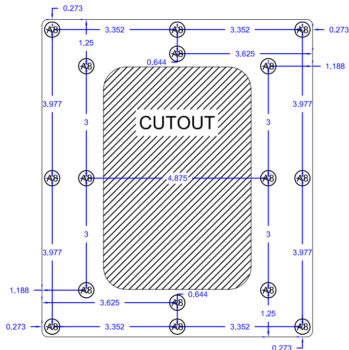
BACK SIDE VIEW OF MAG-KEYPAD-DOOR
