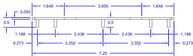
BOTTOM SIDE VIEW OF MAG-KEYPAD-DOOR
