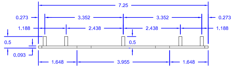
TOP SIDE VIEW OF MAG-KEYPAD-DOOR
