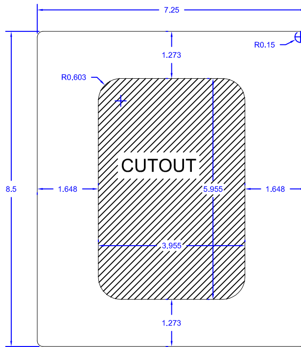
FRONT SIDE VIEW OF MAG-KEYPAD-DOOR
