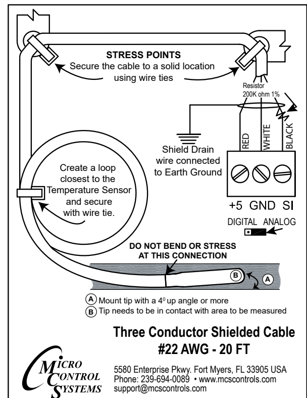
Magnum Sensor Input Wiring Diagram for MCS-T300-L
