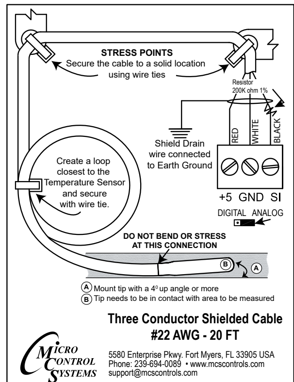
Magnum Sensor Input Wiring Diagram for MCS-T300-L
