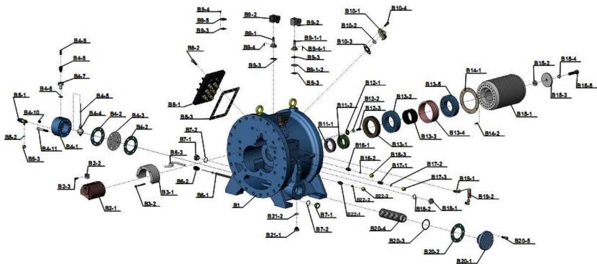
RC2-170~620 Except 180&610 B - Compression Casing
