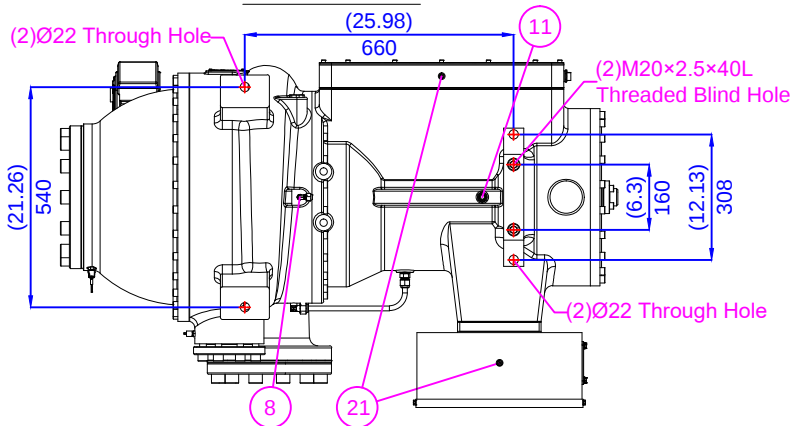
Bottom View
