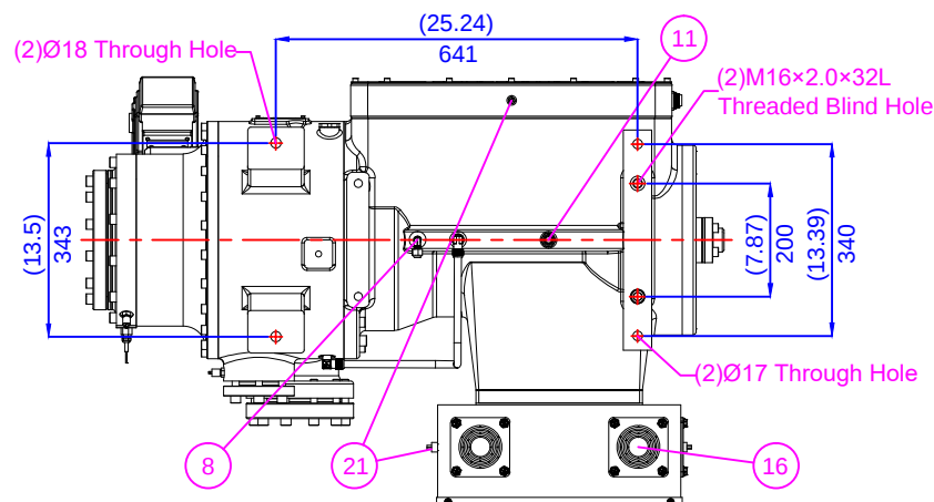
Right View
