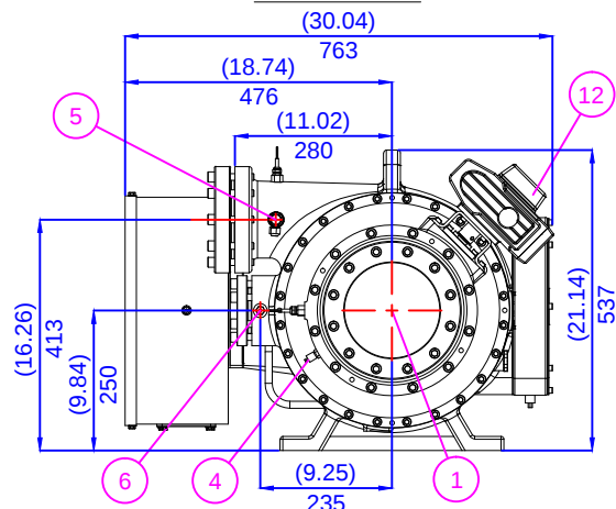
Left View
